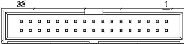
Figure 4. MXP Pinout
